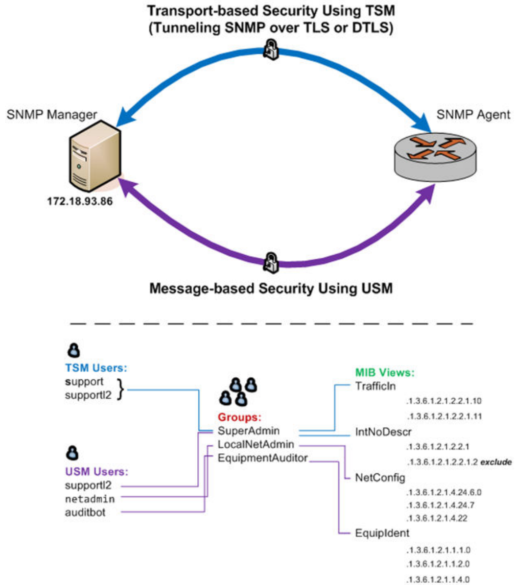
FIGURE 6 SNMPv3 topology example
