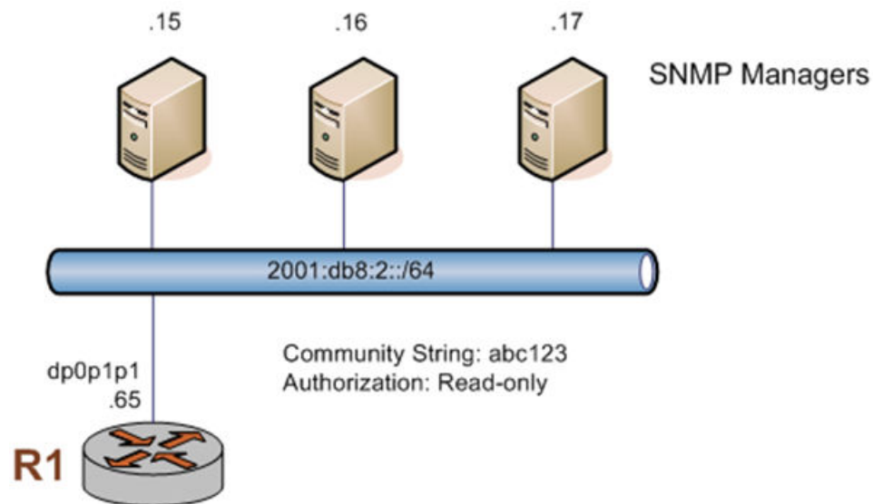
FIGURE 5 Configuring SNMP communities and traps - IPv6
