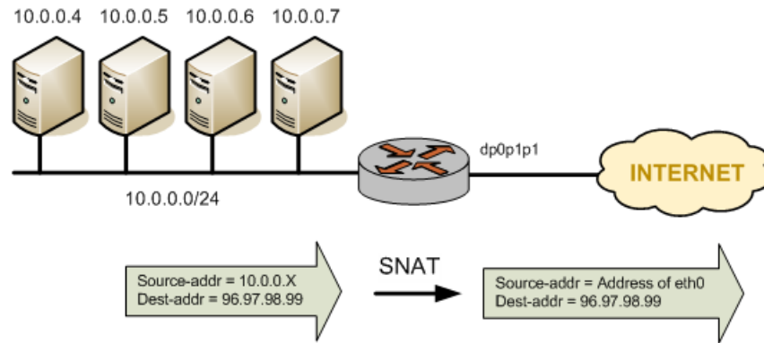
FIGURE 21 Masquerade NAT
