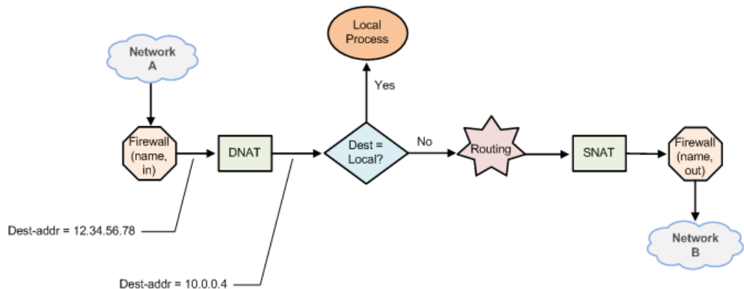
FIGURE 13 Pass-through DNAT firewall decisions
