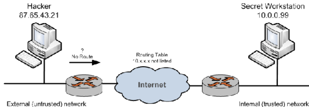
FIGURE 3 NAT combined with firewall
