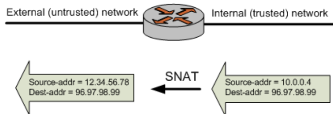
FIGURE 4 Source NAT (SNAT)
