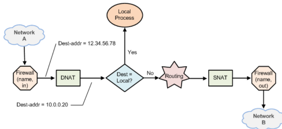
FIGURE 12 Brocade vRouter-destined DNAT routing decisions
