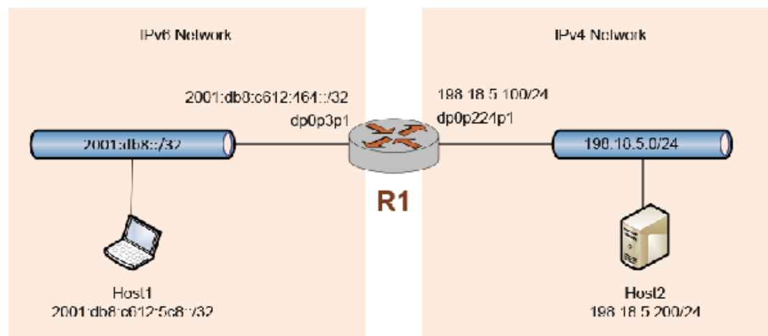
FIGURE 27 NAT 6-4 configuration example
