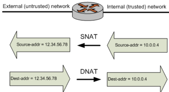
FIGURE 6 Bidirectional NAT
